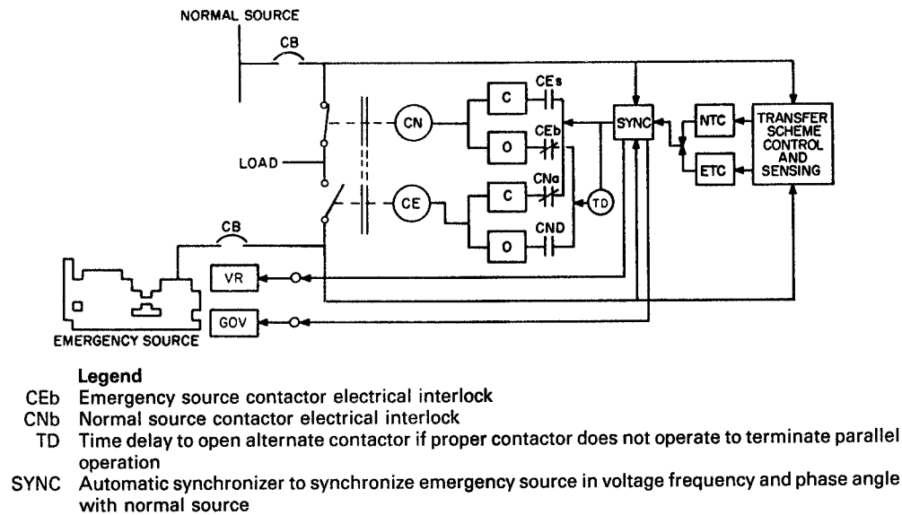
Figure 4-15—Closed transition transfer
